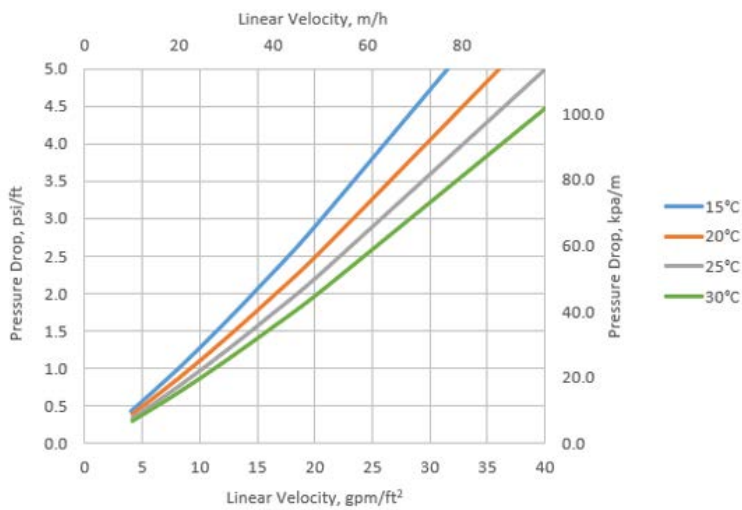
Figure 2 – Pressure drop
