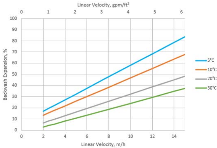
Figure 1 – Backwash expansion
